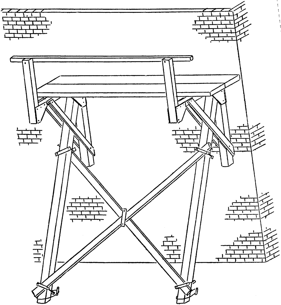
BRACKET SCAFFOLD.
